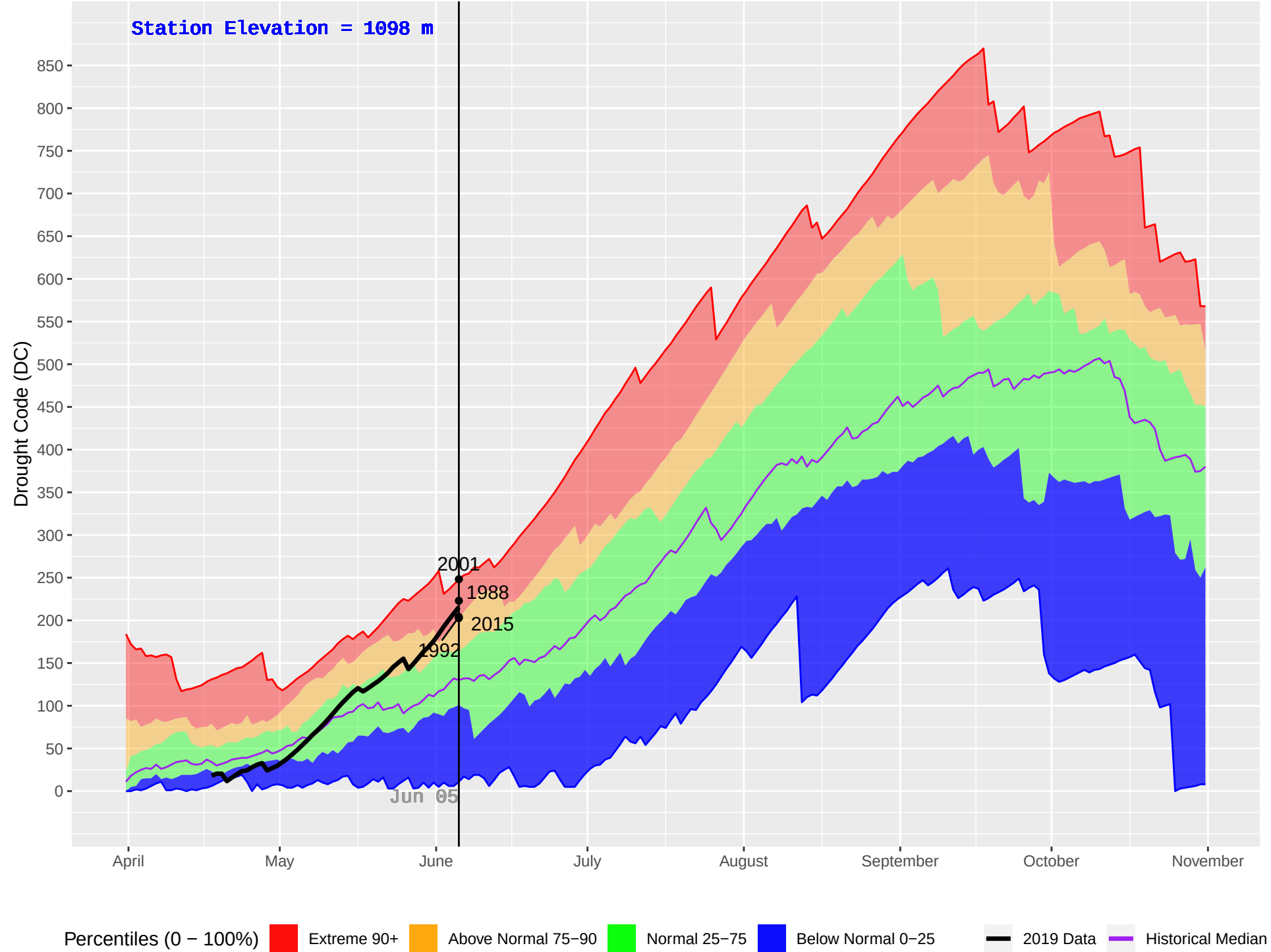
GOATFELL (401) : Historical (1986–2018) and Current (2019) Daily Drought Code (DC)
