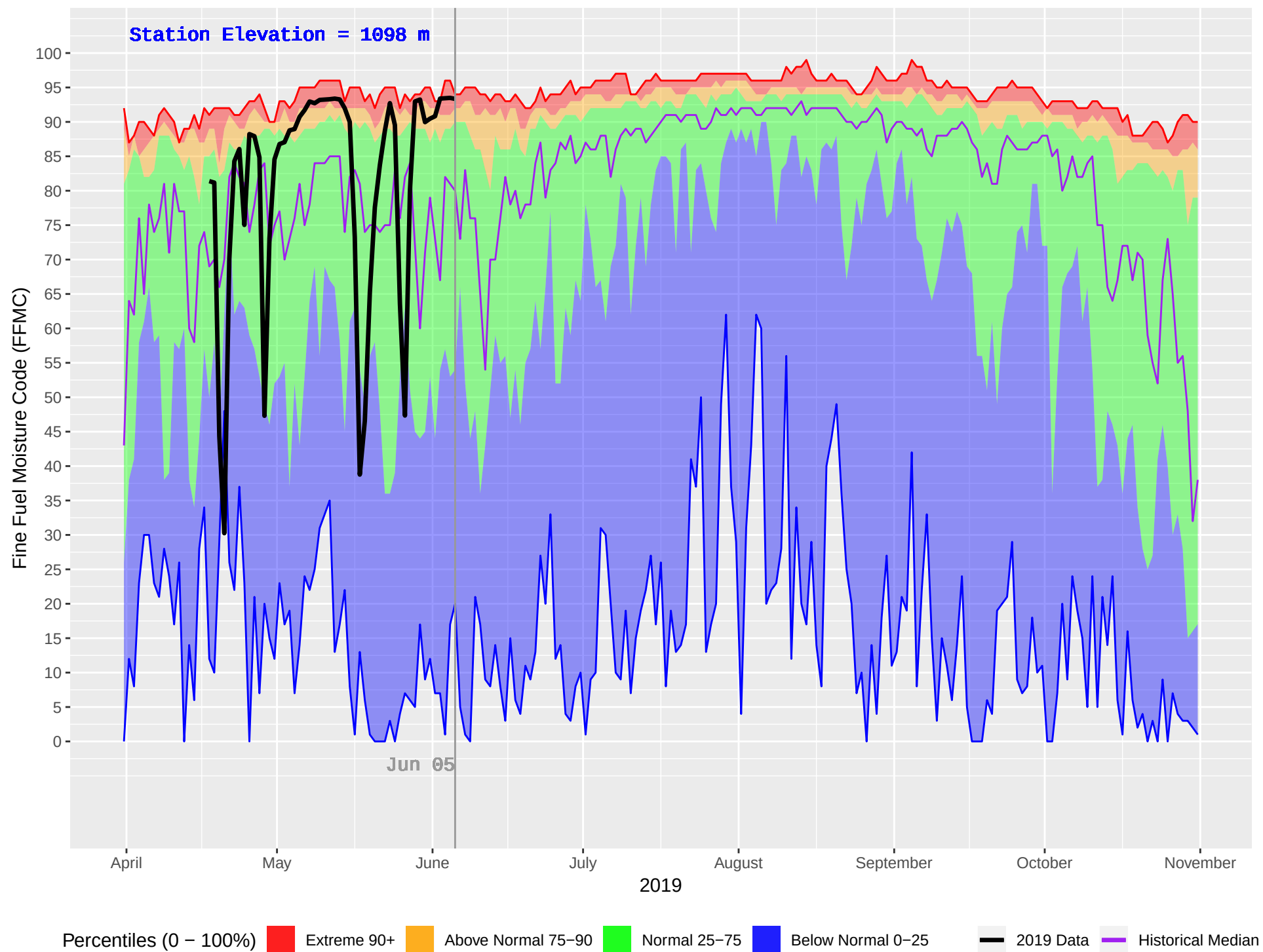
GOATFELL (401) : Historical (1986–2018) and Current (2019) Daily Fine Fuel Moisture Code (FFMC)
