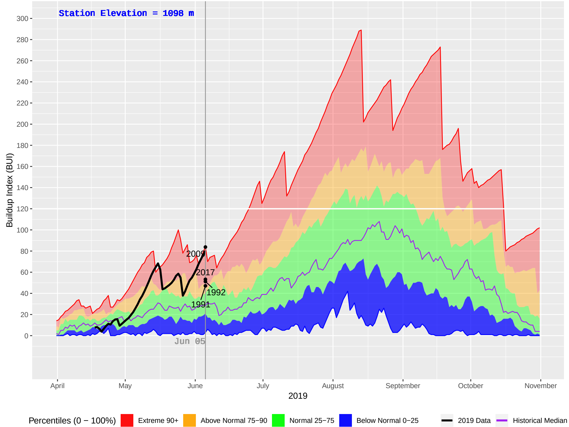
GOATFELL (401) : Historical (1986–2018), Current (2019) Daily Buildup Index (BUI)
