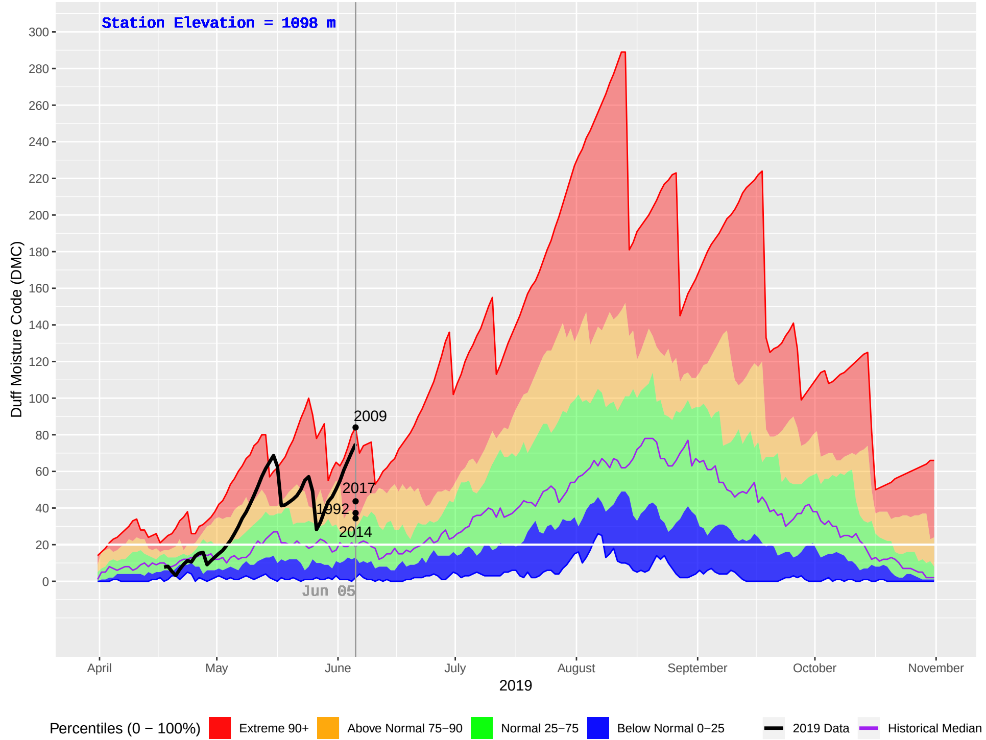
GOATFELL (401) : Historical (1986–2018), Current (2019) Daily Duff Moisture Code (DMC)
