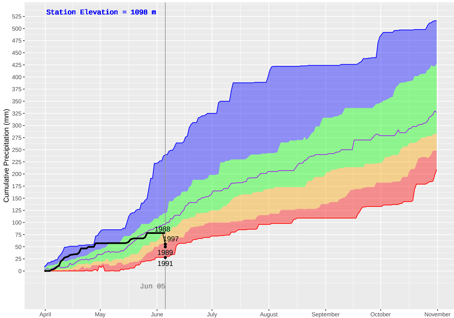
GOATFELL (401) : Historical (1986–2018), Current (2019) Daily Cumulative Precipitation
