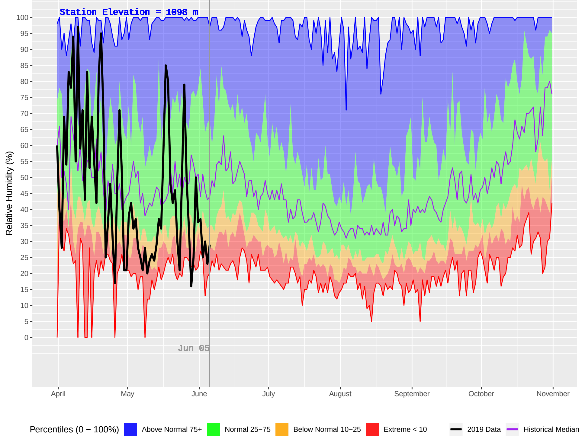
GOATFELL (401) : Historical (1986–2018) and Current (2019) Daily Relative Humidity
